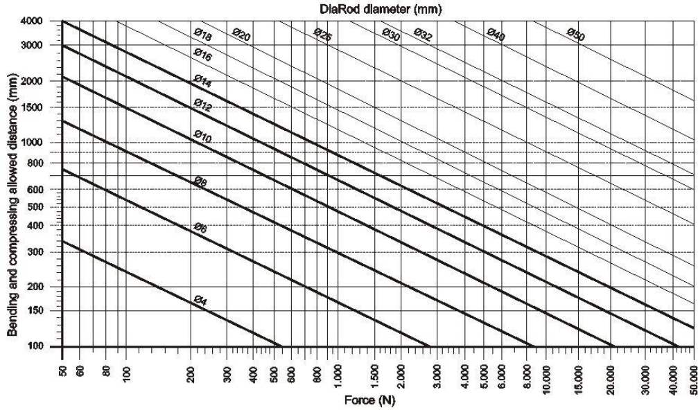
Axial load diagram
