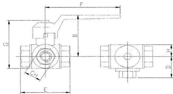
T-Port Configuration
